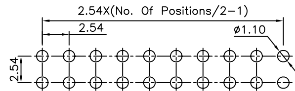
PCB Layout
