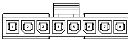
8PIN
