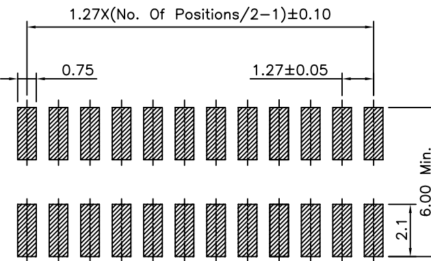
PCB Layout
