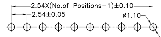
PCB Layout
