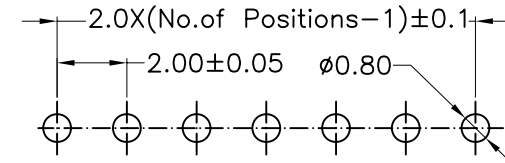
PCB Layout
