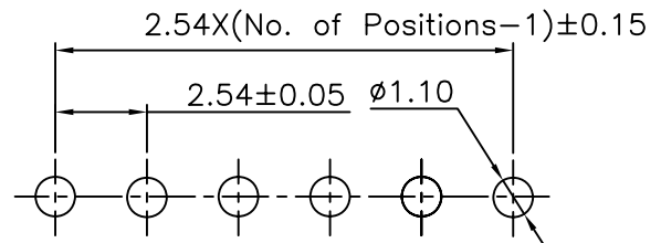
PCB Layout
