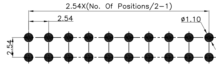
PCB Layout
