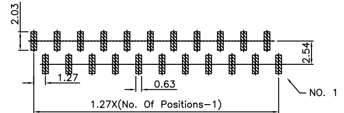
B1 Type PCB Layout
