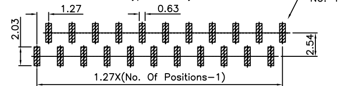
B2 Type PCB Layout
