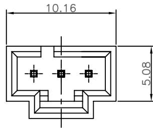
(3 Pin)
