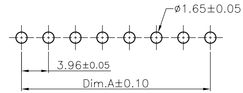
PCB LAYOUT
