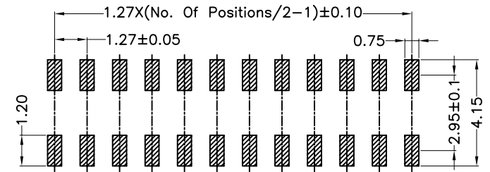
PCB Layout
