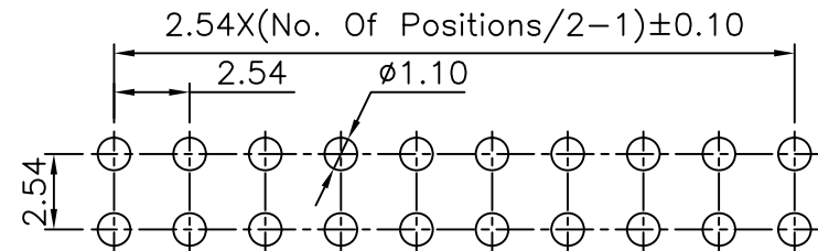
PCB Layout
