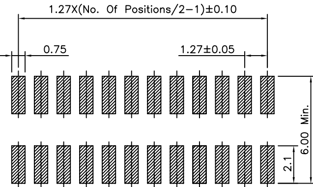
PCB Layout
